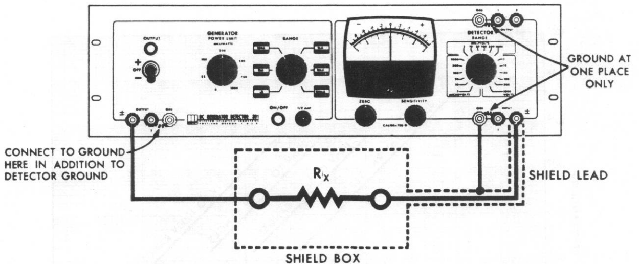
Figure 2.6 High-Resistance Measurement
